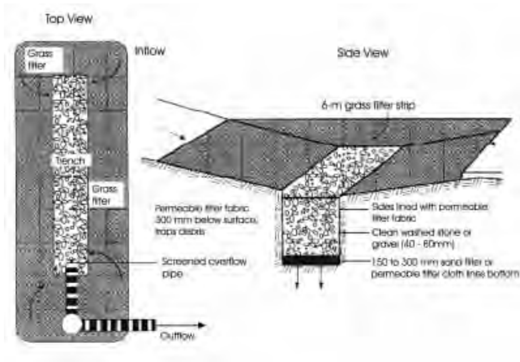
Figure 4-12. Median strip infiltration trench design (adapted from MWCOG, 1987).
