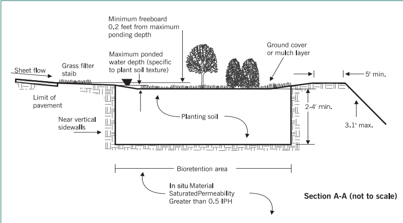
Figure 2-4. Bioretention cell
